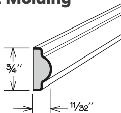
SINGLE BEAD
