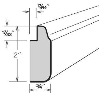
MIRROR
