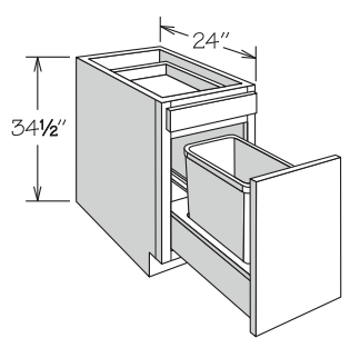
1 WASTEBASKET
