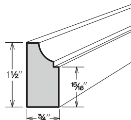
CLASSIC TRIM
