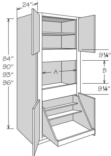
90" High Shown
