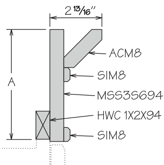
MODERN 200
