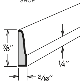
STRAIGHT TRIM
