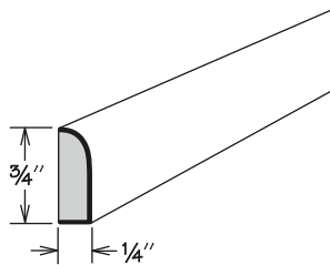
SCRIBE
