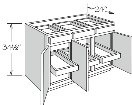
3 SLIDING SHELVES
