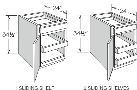
1 SLIDING SHELF
