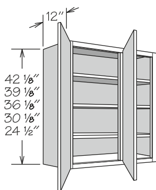
42" High Shown
