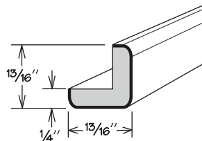
OUTSIDE CORNER
