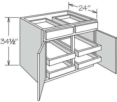
4 SLIDING SHELVES
