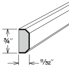
SHAKER
